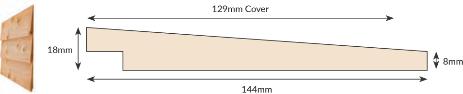
FEATHER EDGE Ex150mm x 22mm PFC009
