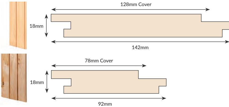
VERTICAL SHADOW GAP Ex150mm x 22mm PFC005 & Ex100mm x22mm PFC006
