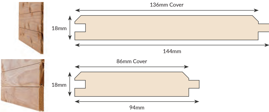
T&G V JOINT Ex150mm x 22mm PFC001 & Ex100mm x22mm PFC002
