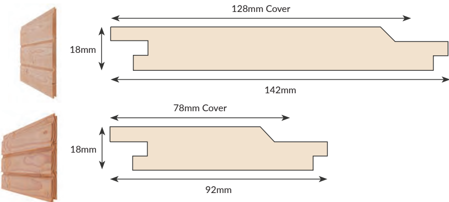
HORIZONTAL SHADOW GAP Ex150mm x 22mm PFC003 & Ex100mm x22mm PFC004
