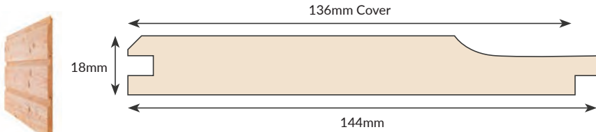
SHIPLAP Ex150mm x22mm PFC008
