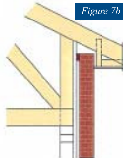
Timber frame
