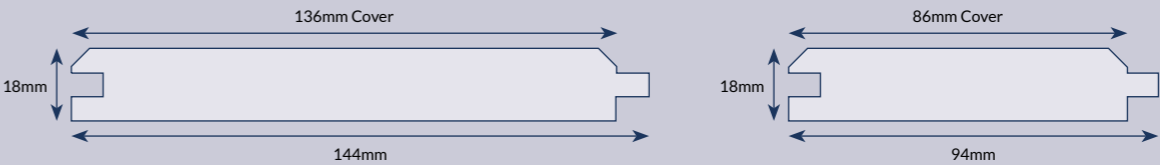
HORIZONTAL SHADOW GAP Ex150mm x 22mm PFC003 & Ex100mm x22mm PFC004
