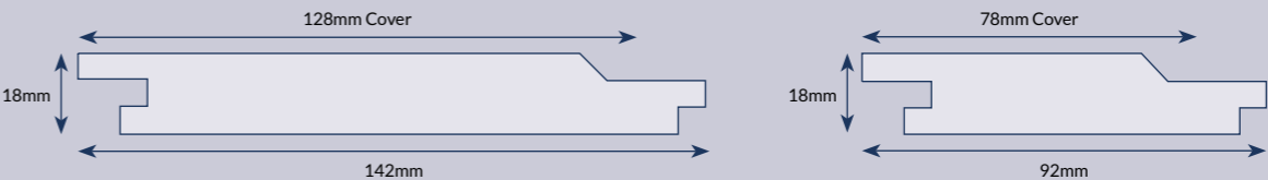
VERTICAL SHADOW GAP Ex150mm x 22mm PFC005 & Ex100mm x22mm PFC006
