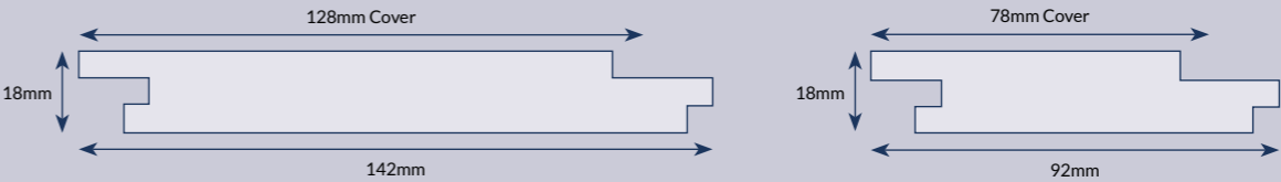
SCREEN Ex150mm x 22mm PFC007
