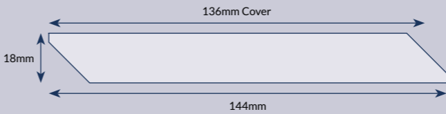
FEATHER EDGE Ex150mm x 22mm PFC009
